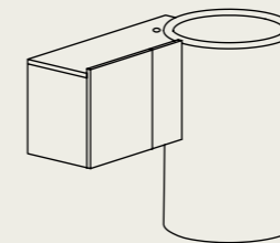
Lavabo freestanding con mobile sospeso 90 destro/sinistro Freestanding washbasin with wall-hung cabinet 90, right / left version cm 57 x 113 x 85 h
