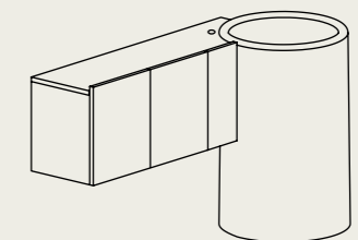
Lavabo freestanding con mobile sospeso 128 destro/sinistro Freestanding washbasin with wall-hung cabinet 128, right / left version cm 57 x 152 x 85 h
