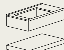
Lavabo con mensola Washbasin with shelf cm 90 x 55 x 21 h (fascione/base unit) cm 90 x 50 x 7 h (mensola/shelf)
