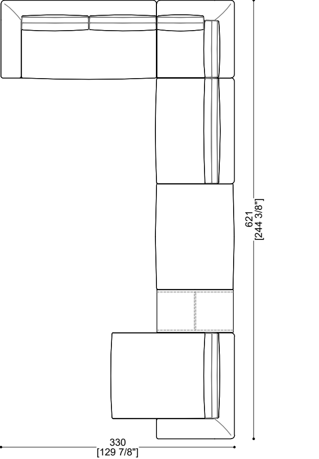
DORIAN COMPOSITION 16 + jolly
