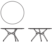
BR_1VS cm. Ø130x73h. inch Ø51"x28"½h.
