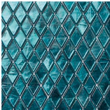
Fluorite
